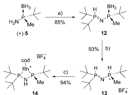
Scheme 5. Synthesis of the aminodiphosphine rhodium complex 14 . Reagents and conditions: a) NaH, t Bu 2 PCL, 60 °C, THF. b) HBF 4 , 65 °C, MeOH. c) [Rh(cod) 2 ] + BF 4 − , Na 2 CO 3 , THF. cod = 1,5-cyclooctadiene.
